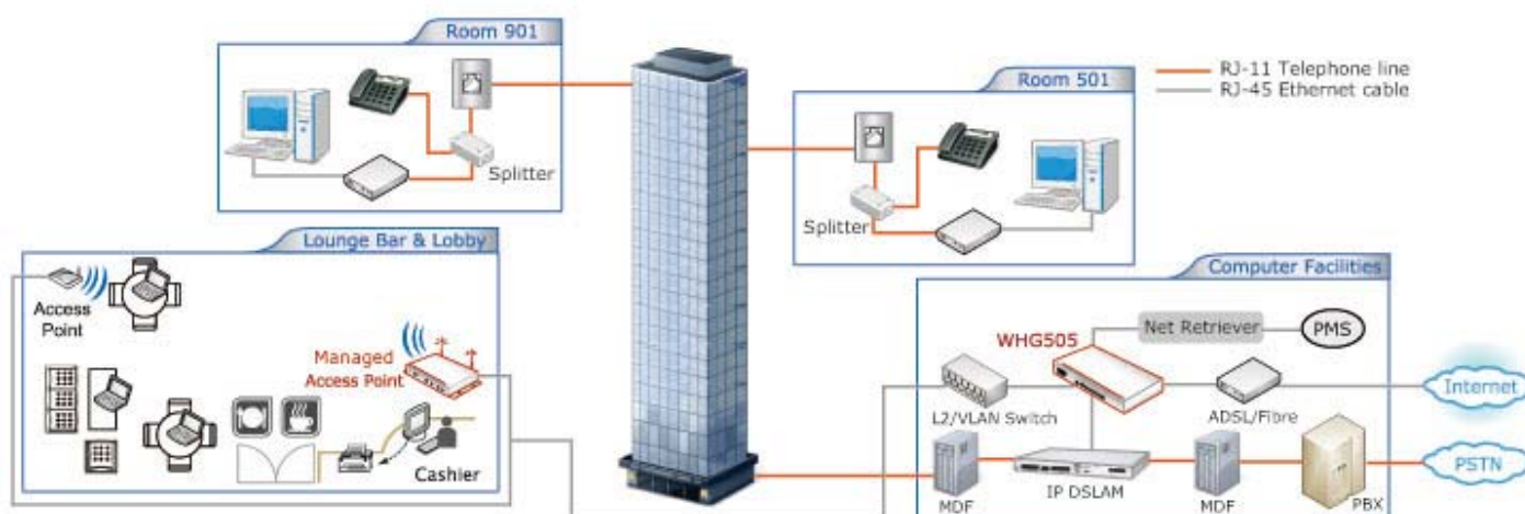
Fig.2. WHG505 in a Hotel - Capable of integrating with DSLAM and PMS
