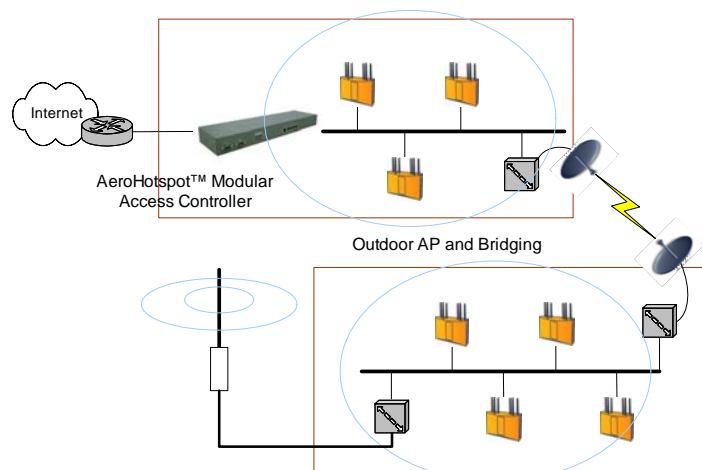
AeroHotspot™ Modular Access Controller with Indoor / Outdoor WLAN Extension
